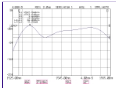
ASE C-Band Light Sources without GFF
